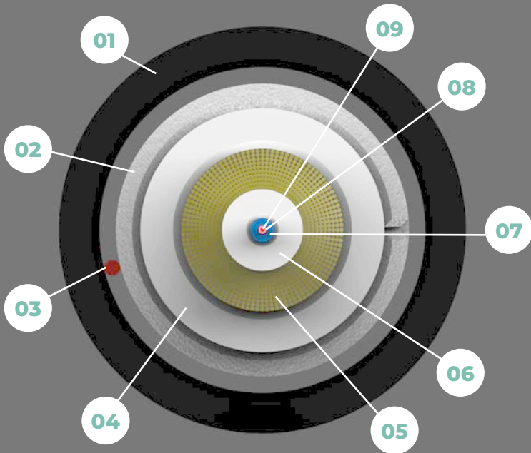
FO Inside/Out - Cable Structure Plan View (Reference PG.1)
